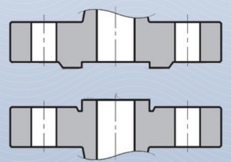
TYPE G AND H - O-RING SPIGOT AND O- GROOVE FACE
